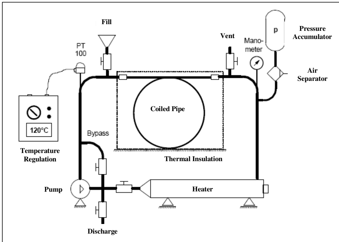
Fig. 1: Schematic plot of the test equipment
