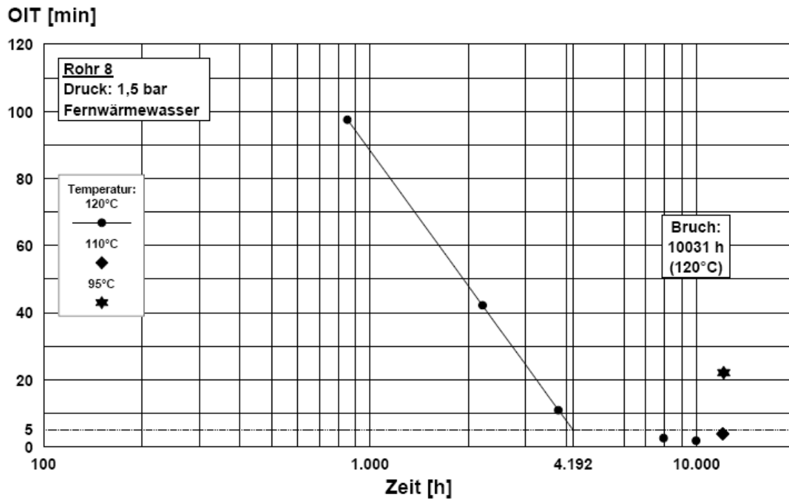
Fig. 3: OIT from pipe # 8 in district heating water
