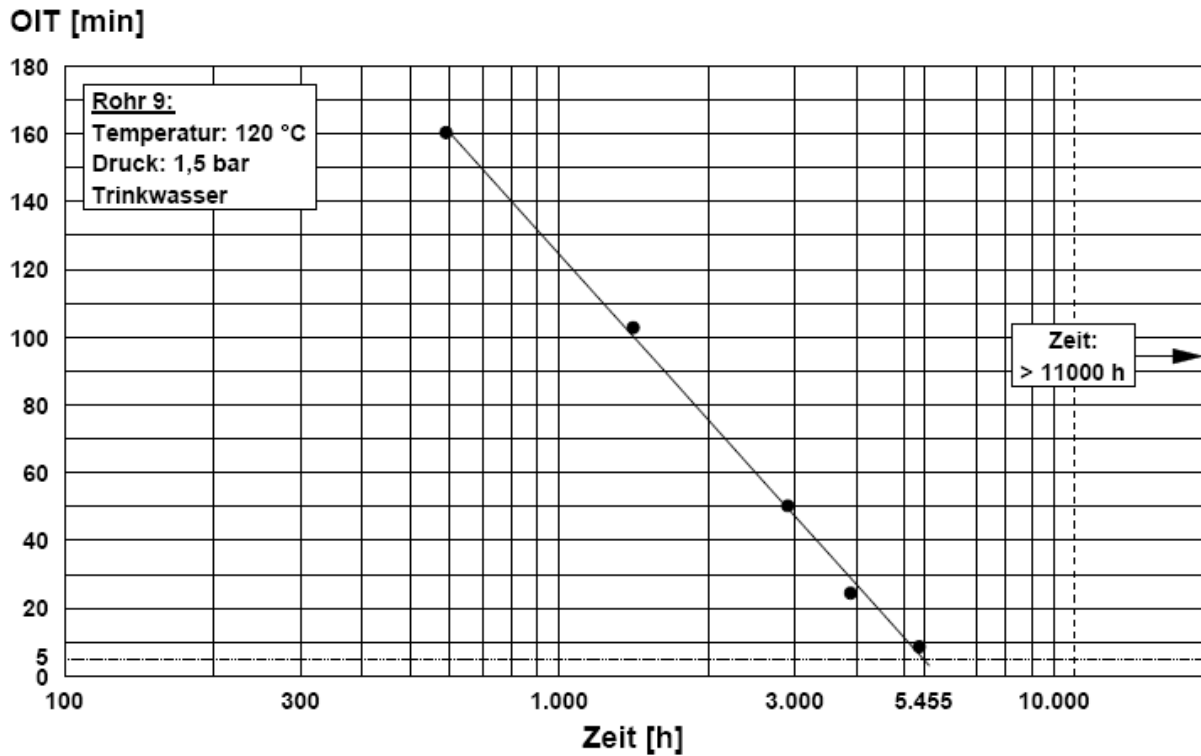
Fig 5: OIT from pipe #9 in drinking water
