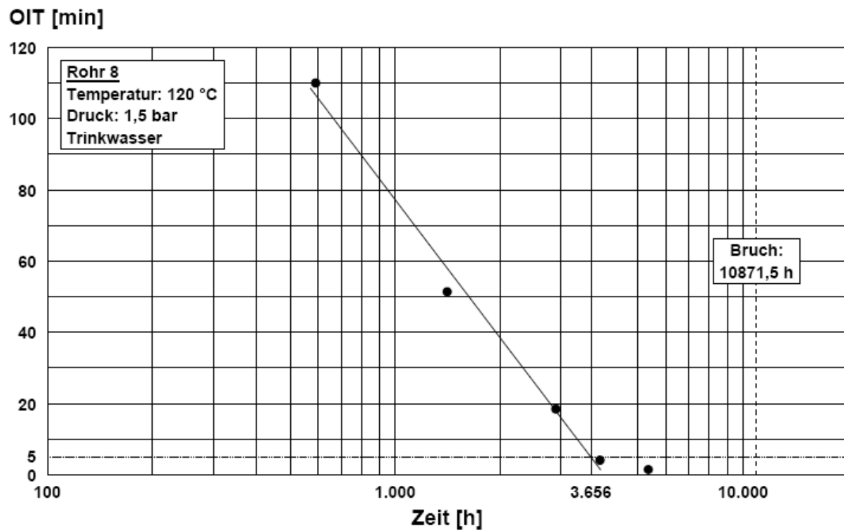
Fig 4: OIT from pipe #8 in drinking water
